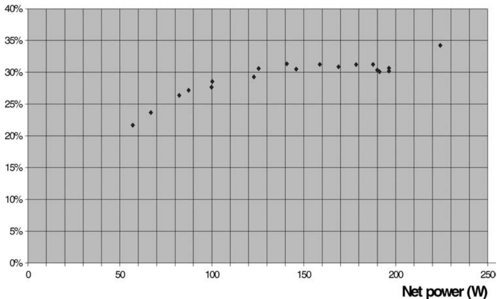
Fig. 3. System efficiency vs. net power.
